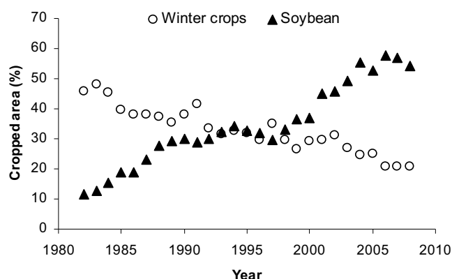
Fig. 1 Percentage of cropped area (period 1982-2008) in the Argentinean Pampas (provinces of Buenos Aires, Córdoba, Entre Ríos, Santa Fe and La Pampa) occupied by soybean and winter crops. Created from published data (SAGPYA 2009).
