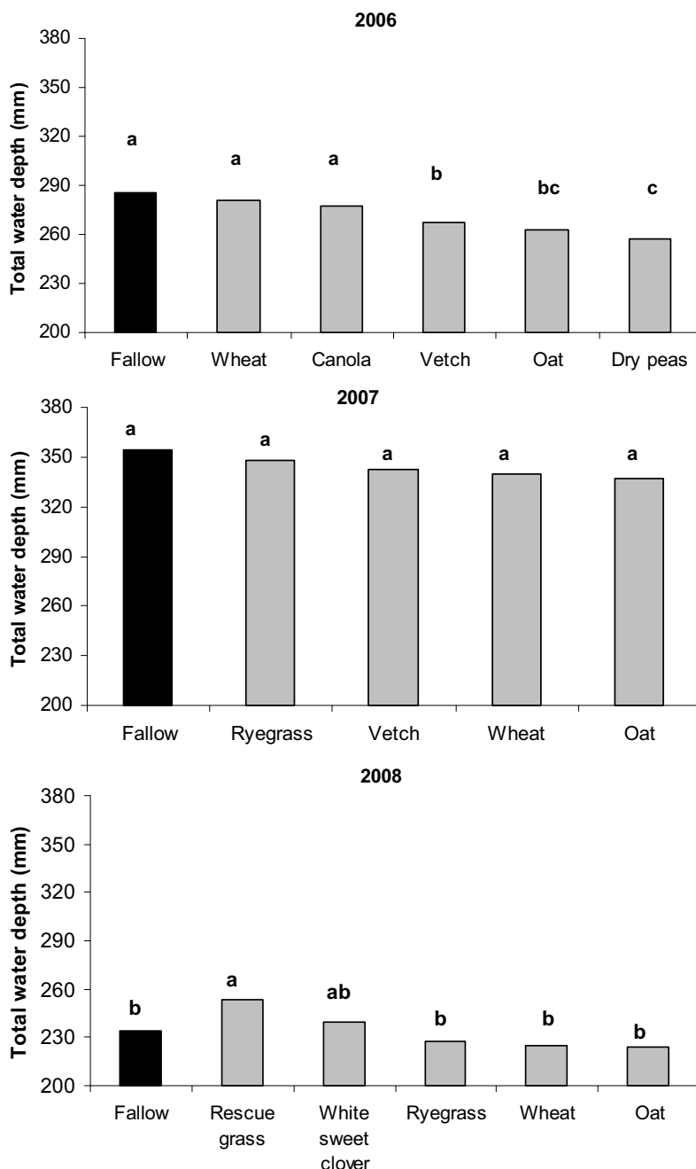
Fig. 2 Total water depth (up to 1 m) in cover crops (unpublished data) at killing date (ca. 20-30 Sept) in the Northern Pampas (Paraná, 32°S; 60°W) from 2006 to 2008. Rescue grass: Bromus catharticus ., White sweet clover: Melilotus alba , Ryegrass: Lolium multiflorum , Wheat: Triticum aestivum , Oat: Avena sativa ., Vetch: Vicia villosa , Canola: Brassica napus , Dry peas: Pisum sativum .
