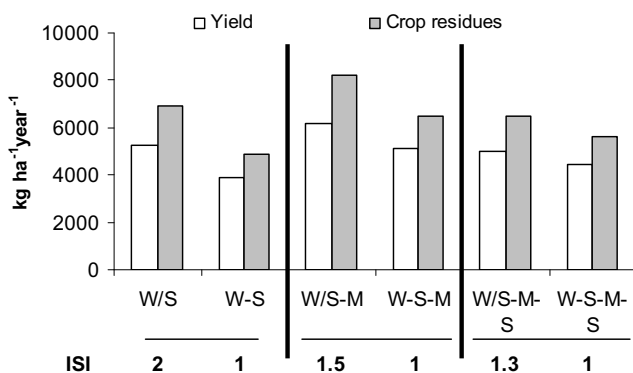
Fig. 6 Annual grain yield and annual crop residues of couple of sequences that differ in intensification level as quantified by ISI (intensification sequence index). Bars represent the average of 30 rotation phases (period 1971-2002) in a simulation study at the Southeastern Pampas (Balcarce, 38°S, 58°W). W: wheat, S: soybean, M: maize; W/S: wheat/soybean double crop. Adapted from Caviglia (2005).
