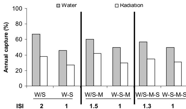
Fig. 5 Water and solar radiation annual capture by couple of sequences that differ in intensification level as quantified by ISI (intensification sequence index). Values expressed as percentage of annual available resources. Bars represent the average of 30 rotation phases (period 1971-2002) in a simulation study at the Southeastern Pampas (Balcarce, 38°S, 58°W). W: wheat, S: soybean, M: maize; W/S: wheat/soybean double crop. Adapted from Caviglia (2005).
